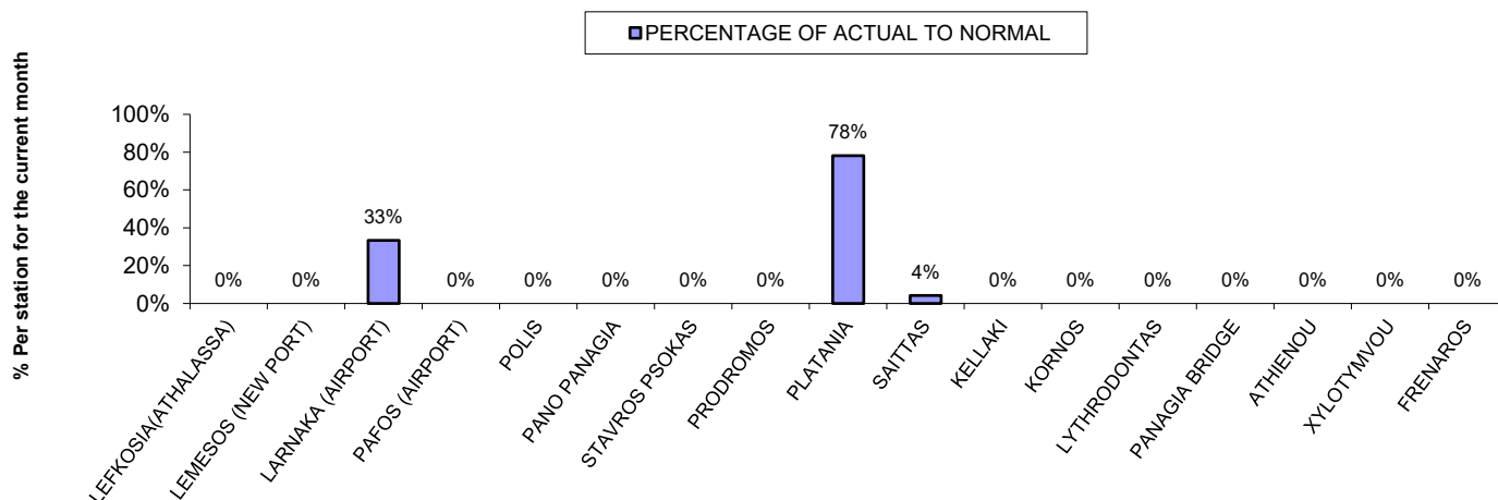
% Rainfall actual to normal until 01/09/2025
